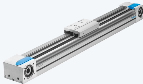
Electric rodless actuator EGC
