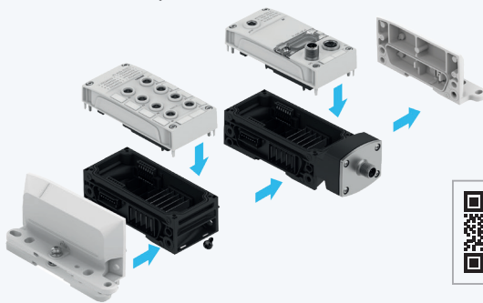
Centralized remote I/O terminals CPX-AP-A
